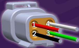
DTM4 Mating Connector Pinout
